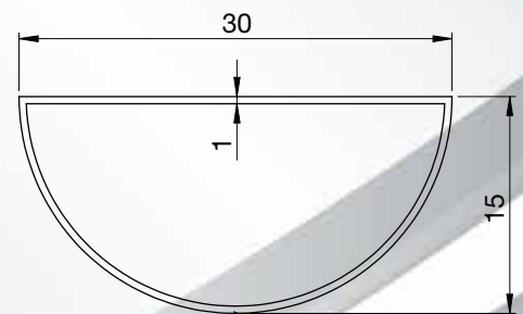
D PROFILE
