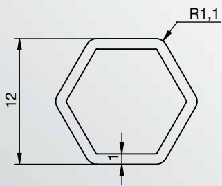
HEXAGON
