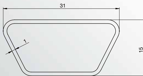
PAN HANDLE
