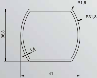
YARI DÜZ OVAL SEMI FLAT OVAL
